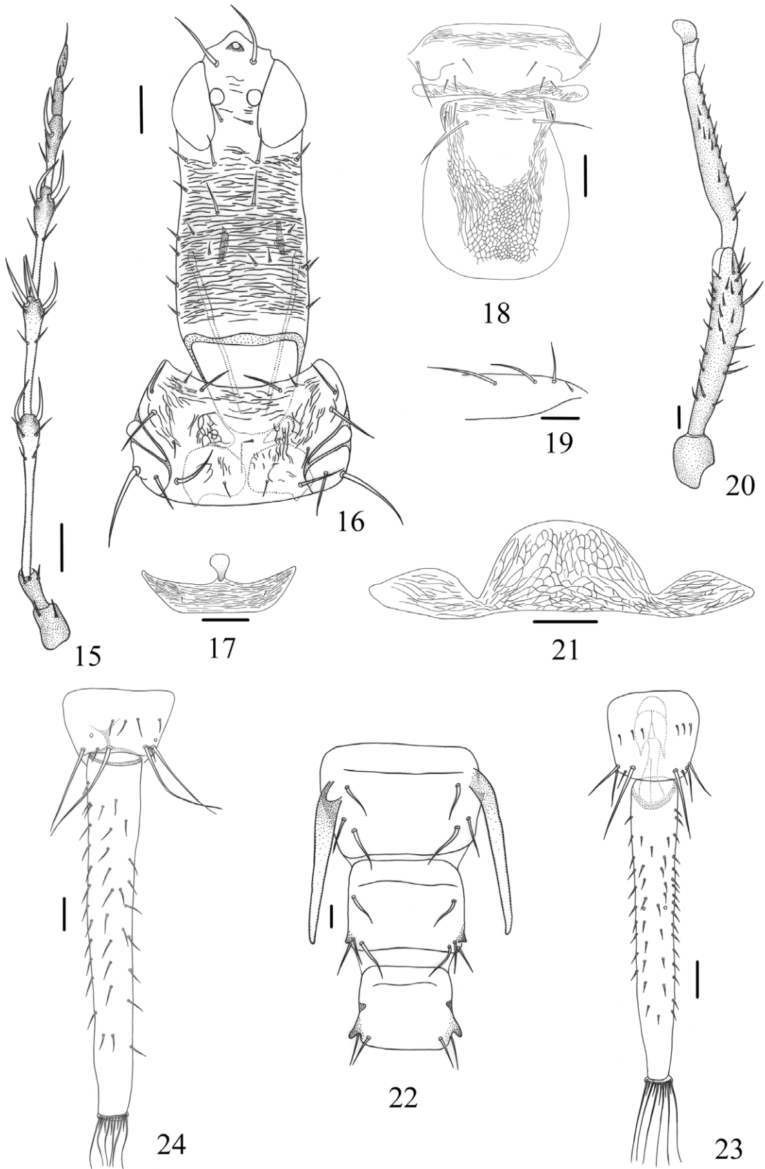
FIGURES 15–24. Bactrothrips furvescрус n. sp. Male: 15 , antenna; 16 , dorsal view of head and pronotum; 17 , mesopraeasterum; 18 , dorsal view of mesonotum and metanotum; 19 , base of forewing; 20 , hind leg; 21 , pelta; 22 , abdominal tergites VI–VIII showing the lateral tubercles; 23 , abdominal tergite IX and tube. Female: 24 , abdominal tergite IX and tube. Scale bars=100µm.
