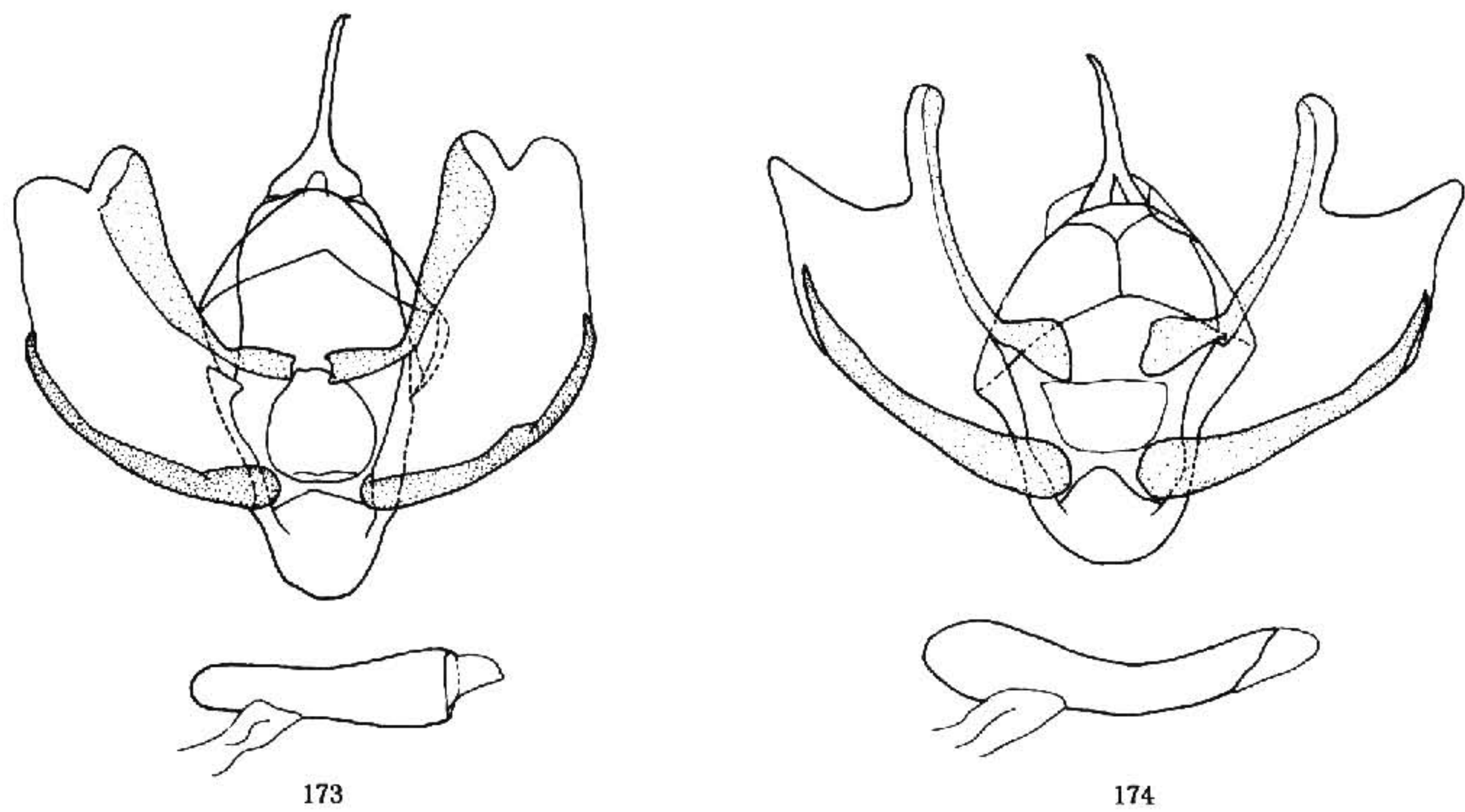
图 173—174 雄性外生殖器. 173. 麻伪沼尺蛾 Nothocasis polystictaria (Hampson); 174. 点脉伪沼尺蛾 N. neurogrammata (Püngeler)
